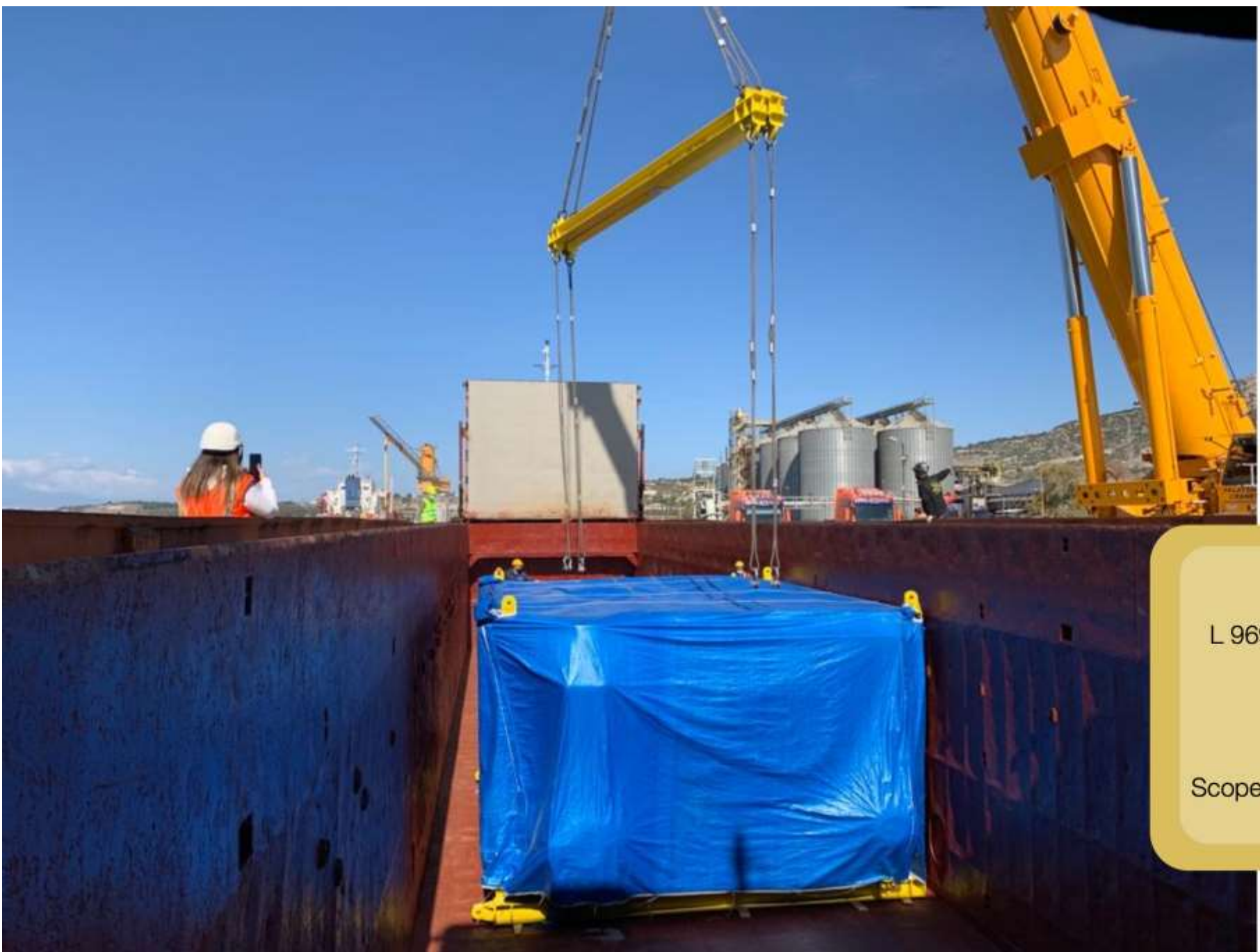
#9 Desalter Drums 2 x 2150x570x485 cm / 80T each Thessaloniki port Scope: FOT till FOB incl lashing,securing
